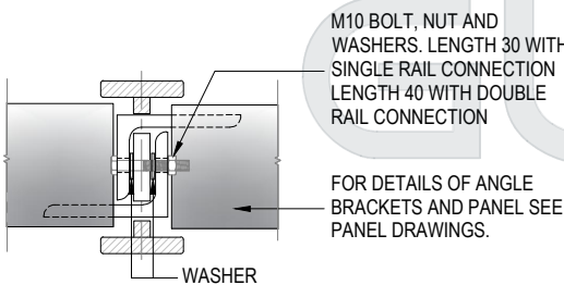
DETAIL OF BOTTOM RAIL CONNECTION
